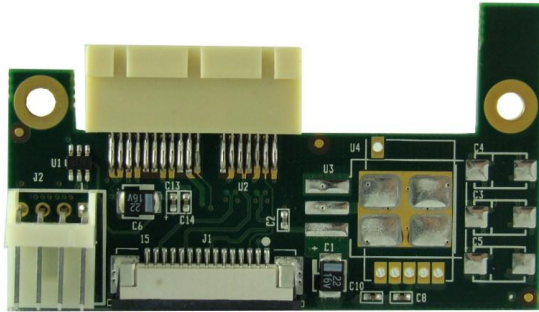
Figure 3: x1 PCI Express adapter board (powered from host card (3.3V only))
