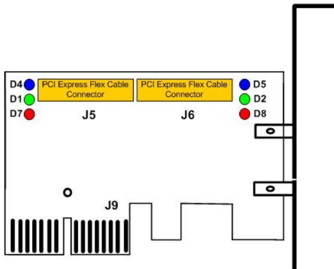
Figure 8: x1 PCI Express Host card layout (bottom side)
