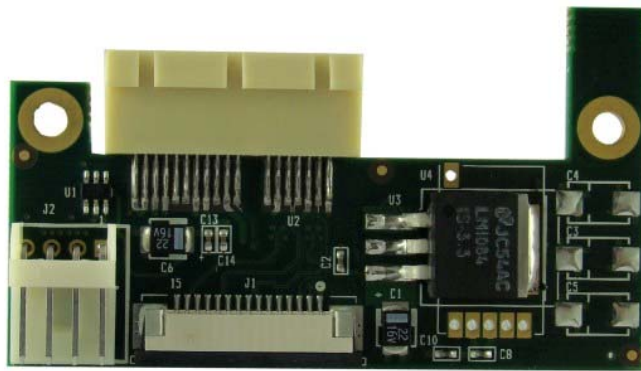
Figure 5: x1 PCI Express adapter board (powered from ATX power supply) (12V, 5V)
