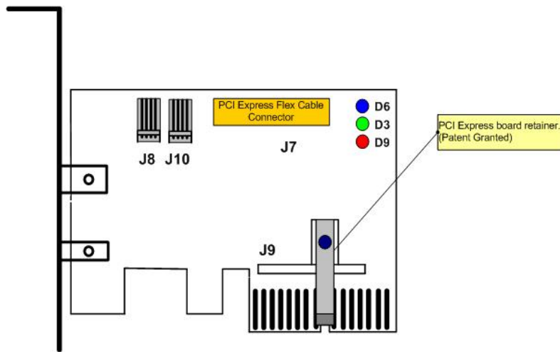
Figure 7: x1 PCI Express Host card layout (top side)
