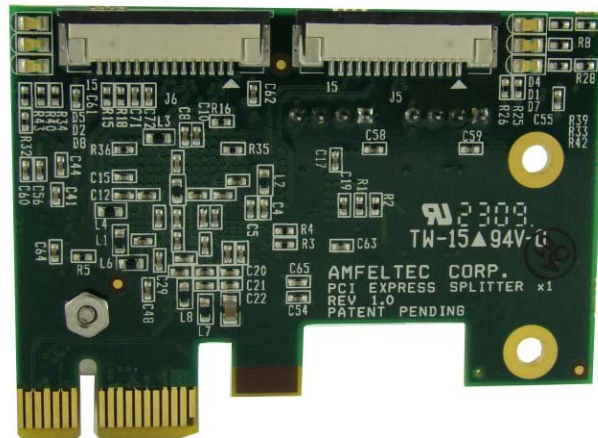
Figure 3: x1 PCI Express Host card (bottom view)
