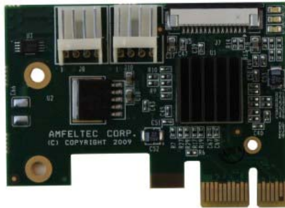
Figure 2: x1 PCI Express Host card (top view)
